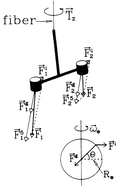
FIG. 2. Forces on a torsion balance located at a latitude \Theta . We assume an attractive composition-dependent force F_5 between the test bodies and the Earth that is stronger for body 1 than for body 2. The possible strength of F_5 has been greatly exaggerated and the magnitude of F^g compared to the inertial force F^i has been reduced by a factor of roughly 100.
