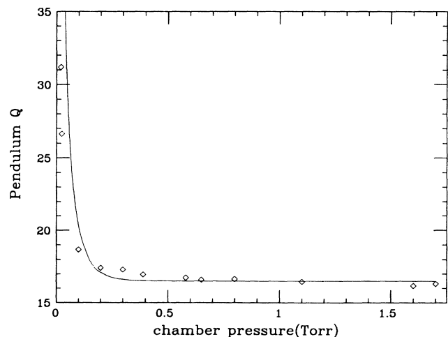
FIG. 5. Pendulum Q as a function of residual gas pressure in the vacuum chamber. Before each equivalence principle data taking cycle, the chamber was evacuated. Data taking did not begin until the pressure had risen to \approx 0.1 Torr.
