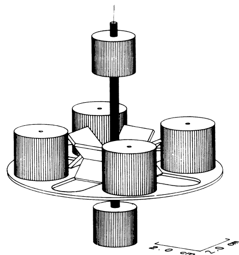
FIG. 4. Scale drawing of the torsion pendulum.
