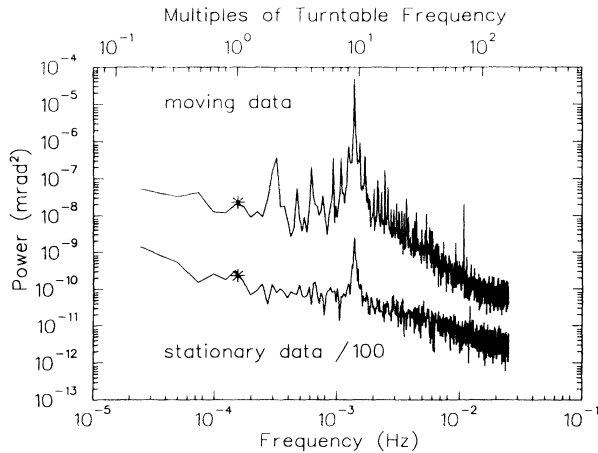
FIG. 19. Power spectrum of the raw difference signal with the apparatus stationary and rotating at n = 9 . Each plot is an average of five equal length ( \approx 11 h) 2048 point transforms. The stationary data have been divided by 100 to separate the two curves. A linear background was subtracted from both sets of raw data before generating the Fourier transform. The two “starred” points at 1\omega represent the scatter in the a(1\omega) coefficients obtained from our standard analysis.
