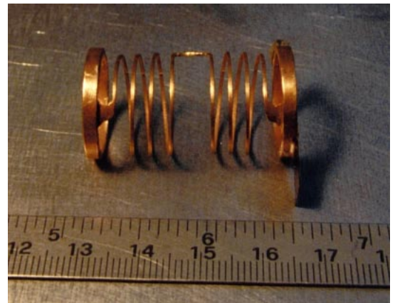
One test body spring: no electric wires Manufactured in CuBe by electroerosion in 3D (DG Technology, Parma)
