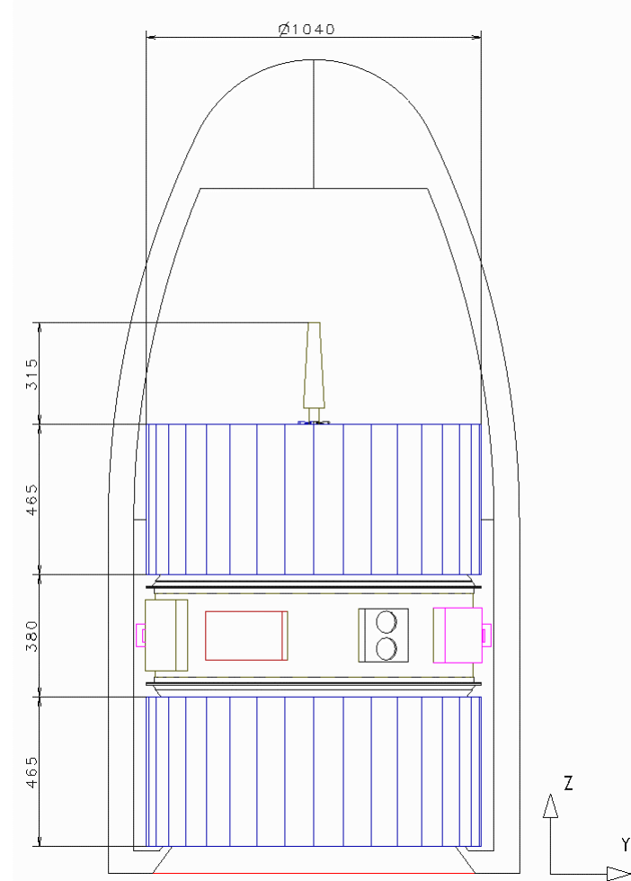
Configuration under the Pegasus fairing
