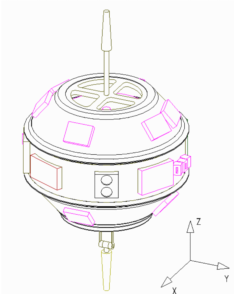
Structural configuration with solar panels removed
