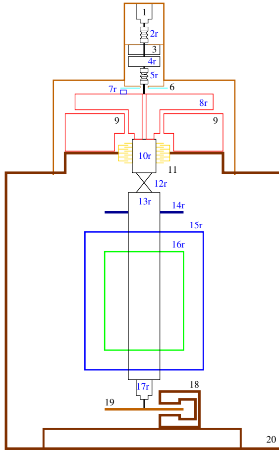
Figure 8: Design for the implementation of the air bearing on GGG. Precision grade ball bearings are manufactured with typical \sim 100 nm geometric tolerances: balls are manufactured with \sim 100 nm sphericity and \sim 500 nm diameter tolerance. Very roughly, a 5 cm diameter ball bearing can then cause a shaft fitted to the inner race to tilt by some \mu\text{rad} . The complexity of the ball bearing result in \simeq \mu\text{rad} shaft tilt noise in the low frequency region of interest for GGG. On the other side, air bearings require very tight bearing gaps for proper operation ( 10\mu\text{m} ) which translates into extremely high accuracy motion with best noise performance. Typical rotary runout can be as low as 1\text{ nm} and tilt characteristics as low as 0.02\mu\text{rad} . Because the air bearing has two surfaces and only two surfaces, the tilt noise is essentially concentrated at the rotation frequency, while the noise performance is order of magnitude better at low frequency. In GGG the air bearing (8r and 9) is intended to allow for the quiet rotation of the shaft (10r) while providing for lateral (due to its cylindrical part) and vertical (due to its planar part) stiffness against forces acting on it. The air bearing requires a small but continuous compressed air flow, so that it has been placed outside the vacuum chamber. The GGG sensitive balance, composed of the two rotating hollow cylindrical test bodies (15r and 16r) differentially coupled in the horizontal plane, is suspended to the 2D flexible joint (12r) with the purpose to insulate this part with respect to terrain tilts and horizontal accelerations. The 2D flexible joint (12r) connects the suspended part of the shaft (13r) to the air bearing rotating part (8r). The ferrofluid vacuum feedthrough (11) allows for the rotational motion transfer to the vacuum inside the chamber. It will be an Hollow Shaft Feedthrough housing the not-suspended part of the GGG shaft (10r). Stiffness against horizontal forces on the shaft (10r) due to the magnets needed by the vacuum feedthrough is provided by the cylindrical part of the air bearing, so that the ball bearing normally used on this type of feedthrough are avoided in this application. The GGG shaft will then be rotating on the air bearing only.
