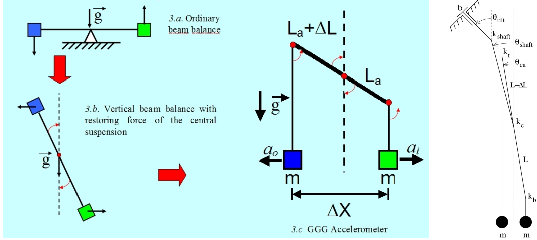
Figure 2: Simplified representation of the GGG balance. (left): The GGG accelerometer is designed to be sensitive to differential forces acting in plane perpendicular to the spin axis, which is in the vertical direction. The two test masses are coupled as in a vertical beam balance with a natural period of differential oscillation relative to each other T_d (see text). (left): The upper part of the shaft, rotating on bearings (b) is tilted by the angle \theta_{tilt} by the terrain and bearings tilt noise; the 2D flexible joint k_{shaft} , placed on the shaft below the bearings, attenuates \theta_{tilt} so that the lower part of the shaft is tilted, at low frequencies, by the attenuated angle \theta_{shaft} = \frac{k_{shaft}}{M_{tot}gL_{shaft}}\theta_{tilt} \ll \theta_{tilt} . The coupling arm (ca) equilibrium position corresponding to the shaft tilt is \theta_{ca} = \frac{k_c}{2mL^2} \frac{T_d^2}{4\pi^2} \theta_{shaft} . Low frequency horizontal acceleration disturbances are equivalent to tilt disturbances ( \Delta a_{horiz-acc} = g\theta_{tilt} )
