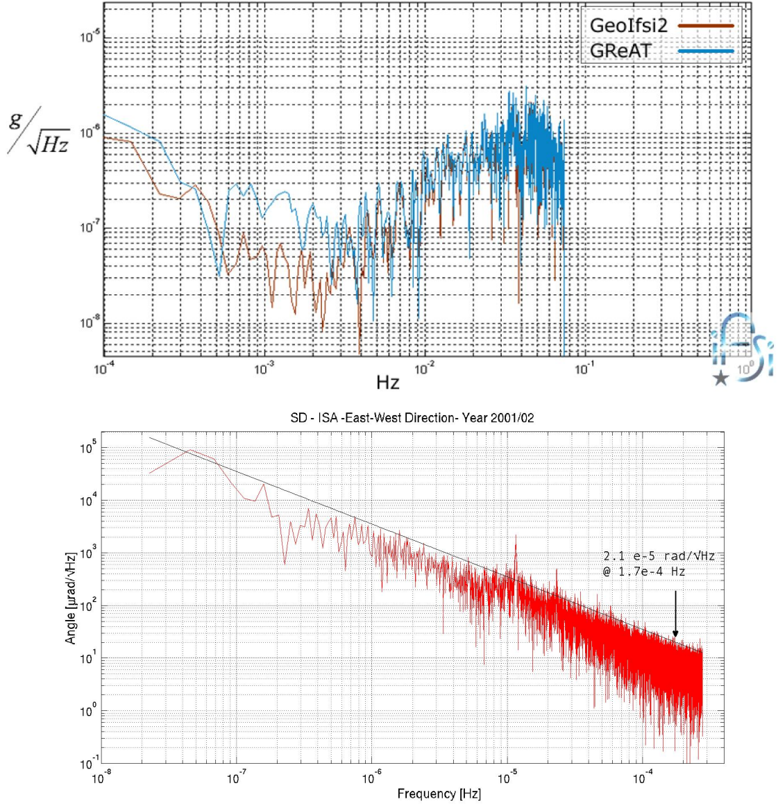
Figure 7: Top: terrain tilt noise as measured by V. Iafolla ISA accelerometer in two different locations at IFSI lab (Roma Tor Vergata) ( g is equivalent to \text{rad} ), showing at the frequency \nu_{GG} = 1.7 \cdot 10^{-4} \text{ Hz} a noise of 9 \cdot 10^{-7} \text{ rad}/\sqrt{\text{Hz}} in a quiet location and of 3 \cdot 10^{-7} \text{ rad}/\sqrt{\text{Hz}} in an underground room. Bottom: terrain tilt noise as measured in Florence (over 16 months) with an ISA tiltmeter, showing 2.1 \cdot 10^{-5} \text{ rad}/\sqrt{\text{Hz}} at \nu_{GG} . In the GGG noise budget we assume for the proposed EGO lab in Cascina (Pisa) a level of terrain tilt noise only a factor 2.5 smaller.
