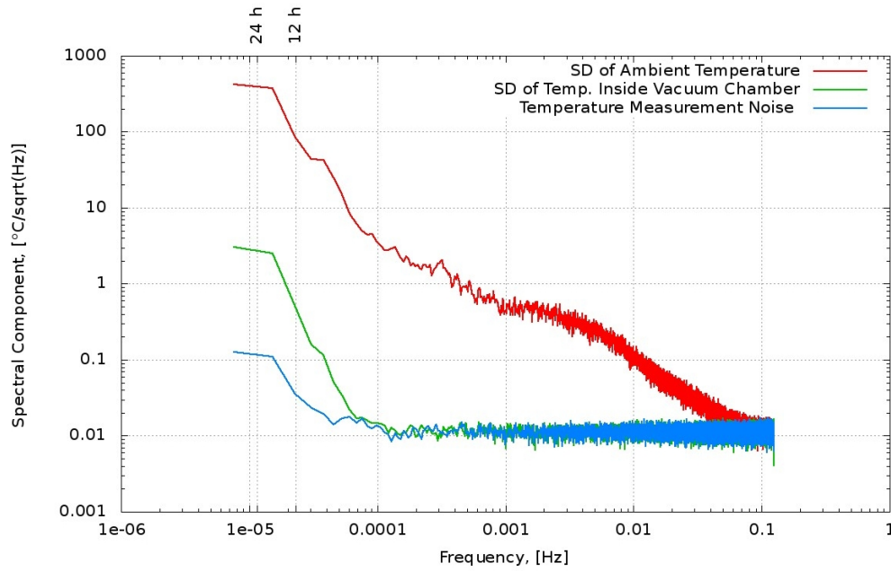
Figure 4: GGG temperature stability relies on a PID (Proportional Integral Derivative), heating only, temperature control acting on the temperature of the vacuum chamber walls. Ambient temperature variations (red curve) are attenuated inside the vacuum chamber (green curve) by about two orders of magnitude, limited only by the temperature readout noise at frequencies higher than 10^{-4} Hz.
