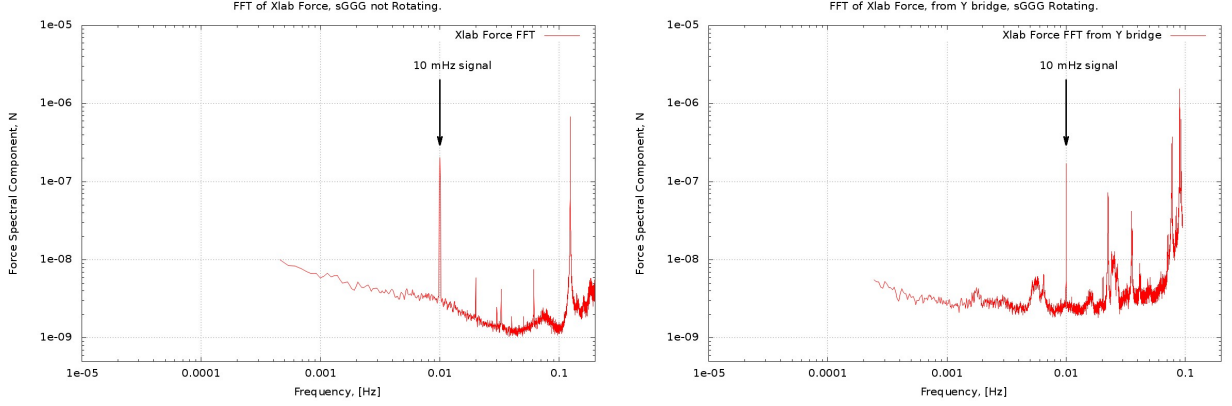
Figure 1: We have experimentally demonstrated that in a 2D oscillator in supercritical rotation like GGG modulation of low frequencies signals at frequencies above resonance is possible without signal attenuation. Left plot: GGG is not rotating and a differential force signal at 0.01 Hz is applied to the test cylinders along the X direction of the horizontal plane of the lab. In this direction the natural frequency of oscillation (resonance) of the test cylinders relative to each other is \nu_x = 0.124 Hz, thus the force is applied below the resonance. We add that the natural oscillation frequency in the perpendicular direction is \nu_y = 0.063 Hz. Right plot: GAG has been set in rotation at \nu_{spin} = 0.19 Hz, the natural oscillation frequency (resonance) during rotation is \nu_w = \sqrt{(\nu_x^2 + \nu_y^2)/2} = 0.098 Hz and the same force signal is applied, which is up-converted close to the spin frequency and therefore at frequencies well above the GGG natural one. The experimental data –i.e. the relative displacements of the test cylinders as given by one of the rotating capacitance bridges which read this differential displacements of the test cylinders– have been demodulated back to the non rotating horizontal plane of the lab for comparison with non rotating case shown above along the X direction. If GGG were an oscillator in 1-D only, a similar rotation of the oscillator above its natural frequency would have been attenuated the signal by a factor 2.56. We note in passing that in the non rotating case (top plot) readout electronics noise increases at lower frequencies as expected, while in the rotating case the relevant readout electronics noise is that at the rotation (that is at the modulation ) frequency.
