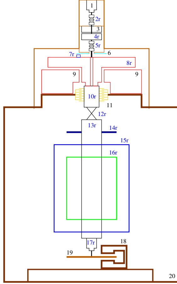
Figure 8: Design for the implementation of the air bearing on GGG. Precision grade ball bearings are manufactured with typical \sim 100 nm geometric tolerances: balls are manufactured with \sim 100 nm sphericity and \sim 500 nm diameter tolerance. Very roughly, a 5 cm diameter ball bearing can then cause a shaft fitted to the inner race to tilt by some \mu\text{rad} . The complexity of the ball bearing result in \simeq \mu\text{rad} shaft tilt noise in the low frequency region of interest for GGG. On the other side, air bearings require very tight bearing gaps for proper operation ( 10\ \mu\text{m} ) which translates into extremely high accuracy motion with best noise performance. Typical rotary runout can be as low as 1\ \text{nm} and tilt characteristics as low as 0.02\ \mu\text{rad} . Because the air bearing has two surfaces and only two surfaces, the tilt noise is essentially concentrated at the rotation frequency, while the noise performance is order of magnitude better at low frequency. In GGG the air bearing (8r and 9) is intended to allow for the quiet rotation of the shaft (10r) while providing for lateral (due to its cylindrical part) and vertical (due to its planar part) stiffness against forces acting on it. The air bearing requires a small but continuous compressed air flow, so that it has been placed outside the vacuum chamber. The GGG sensitive balance, composed of the two rotating hollow cylindrical test bodies (15r and 16r) differentially coupled in the horizontal plane, is suspended to the 2D flexible joint (12r) with the purpose to insulate this part with respect to terrain tilts and horizontal accelerations. The 2D flexible joint (12r) connects the suspended part of the shaft (13r) to the air bearing rotating part (8r). The ferrofluid vacuum feedthrough (11) allows for the rotational motion transfer to the vacuum inside the chamber. It will be an Hollow Shaft Feedthrough housing the not-suspended part of the GGG shaft (10r). Stiffness against horizontal forces on the shaft (10r) due to the magnets needed by the vacuum feedthrough is provided by the cylindrical part of the air bearing, so that the ball bearing normally used on this type of feedthrough are avoided in this application. The GGG shaft will then be rotating on the air bearing only.
