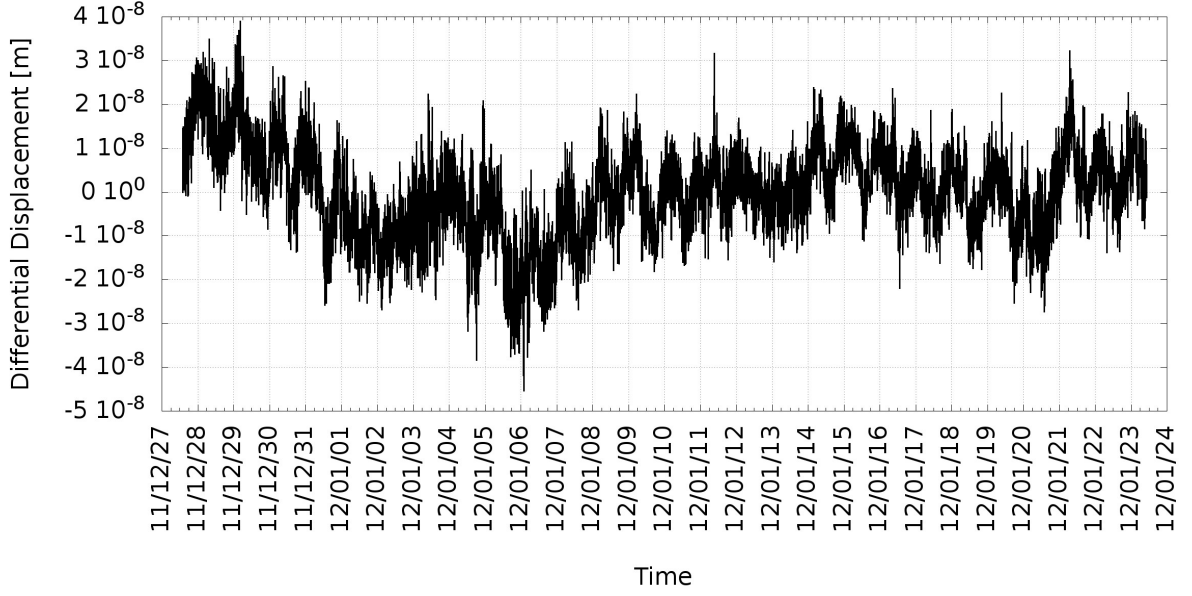
Figure 5: Time series of the relative displacements of the GGG test masses (frequencies above \nu_{cut} = 1 mHz filtered out) in one direction of the horizontal plane of the lab during the ongoing run for a timespan T_{meas} \simeq 28 d. We have analyzed all data collected till 24 January 2012 – 1 day before the closing date for this proposal
